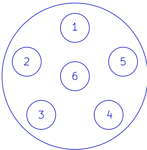
TOP VIEW LOOKING INTO BATTERY CONNECTOR
